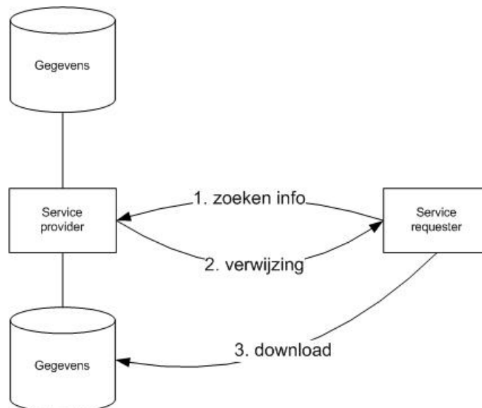
Figuur 2 Use case 'Download'
